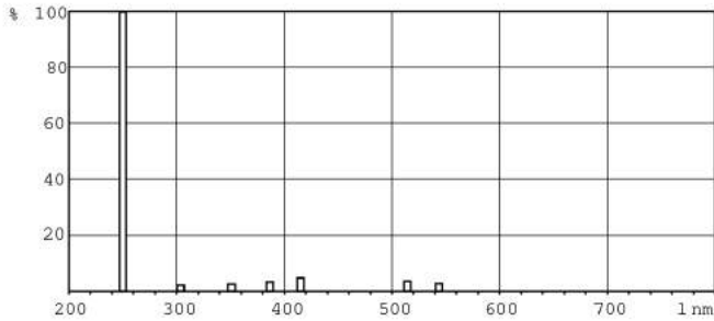
XDPB_XUTUVTLTD-Spectral power distribution B/W
