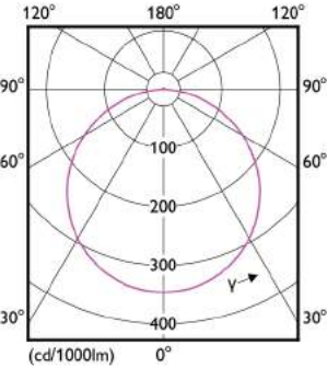
Downlight DN020 G3 CW 7W D125 GM
